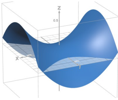
Image: Saddle stationary point. Heuristically, contours are usually
